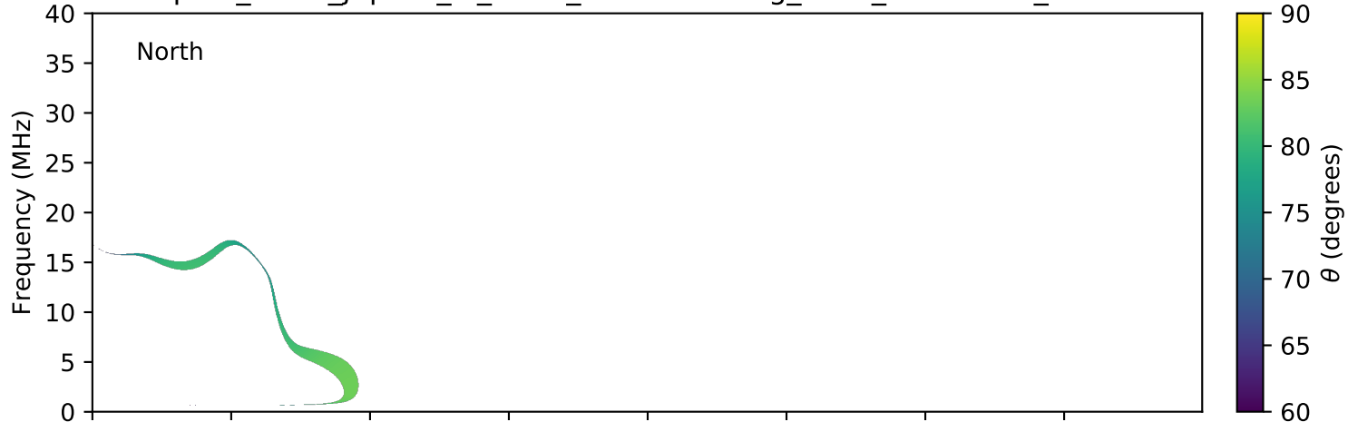
expres_earth_jupiter_io_isaac_lossc-wid1deg_3kev_20090329_v01.cdf
