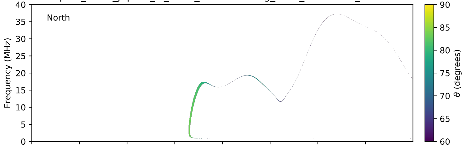
expres_earth_jupiter_io_isaac_lossc-wid1deg_3kev_20090328_v01.cdf
