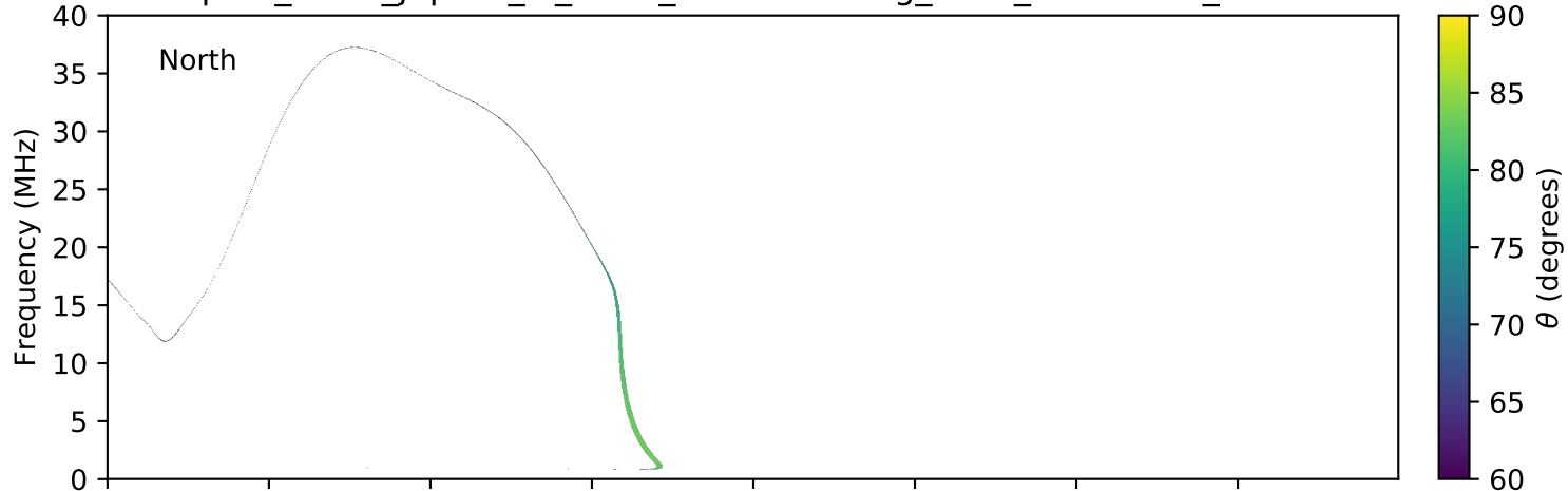
expres_earth_jupiter_io_isaac_lossc-wid1deg_3kev_20090327_v01.cdf
