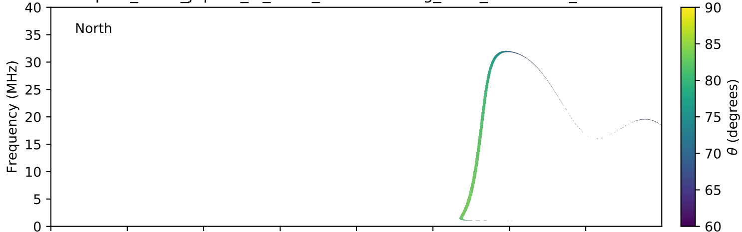
expres_earth_jupiter_io_isaac_lossc-wid1deg_3kev_20090326_v01.cdf
