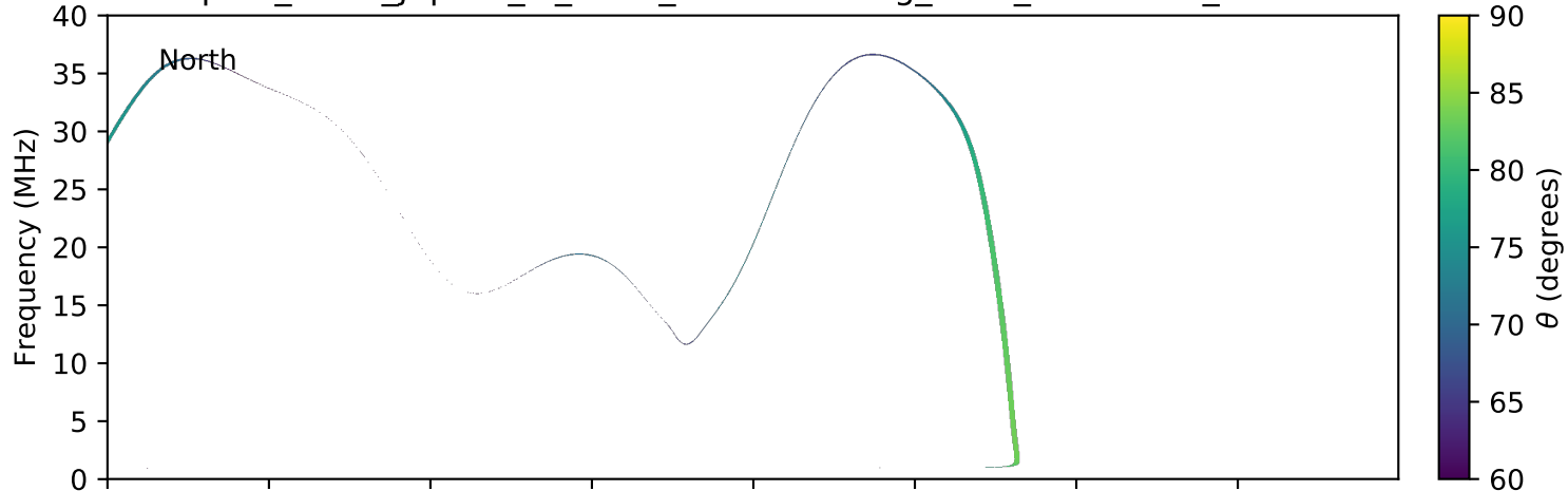
expres_earth_jupiter_io_isaac_lossc-wid1deg_3kev_20090325_v01.cdf
