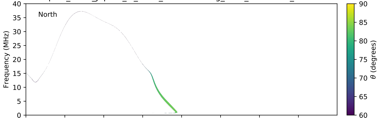
expres_earth_jupiter_io_isaac_lossc-wid1deg_3kev_20090311_v01.cdf
