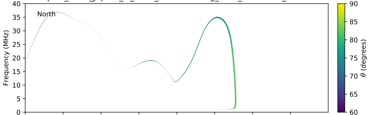
expres_earth_jupiter_io_isaac_lossc-wid1deg_3kev_20090302_v01.cdf
