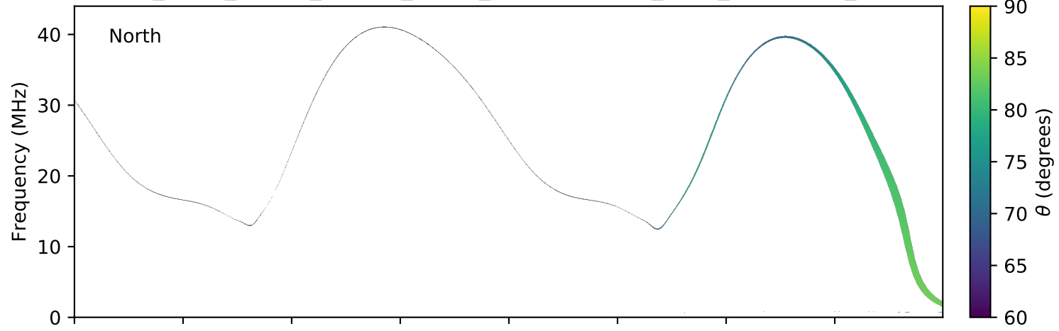
expres_earth_jupiter_europa_jrm09_lossc-wid1deg_3kev_20090320_v01.cdf
