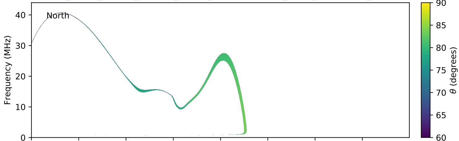
expres_earth_jupiter_europa_jrm09_lossc-wid1deg_3kev_20090317_v01.cdf
