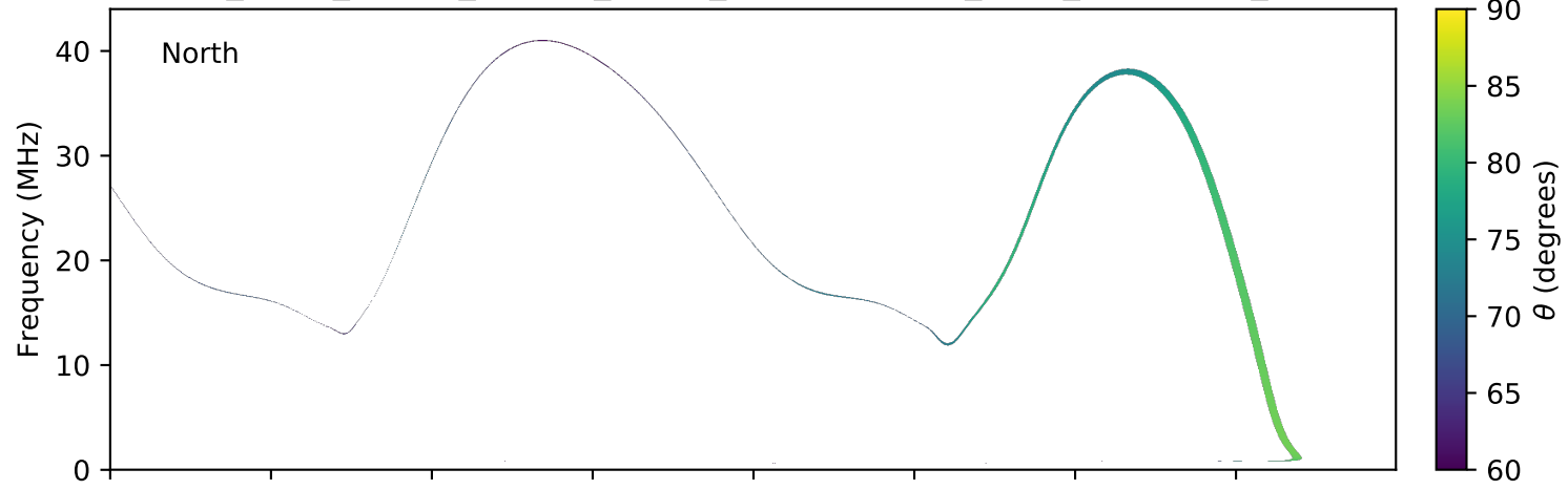
expres_earth_jupiter_europa_jrm09_lossc-wid1deg_3kev_20090313_v01.cdf
