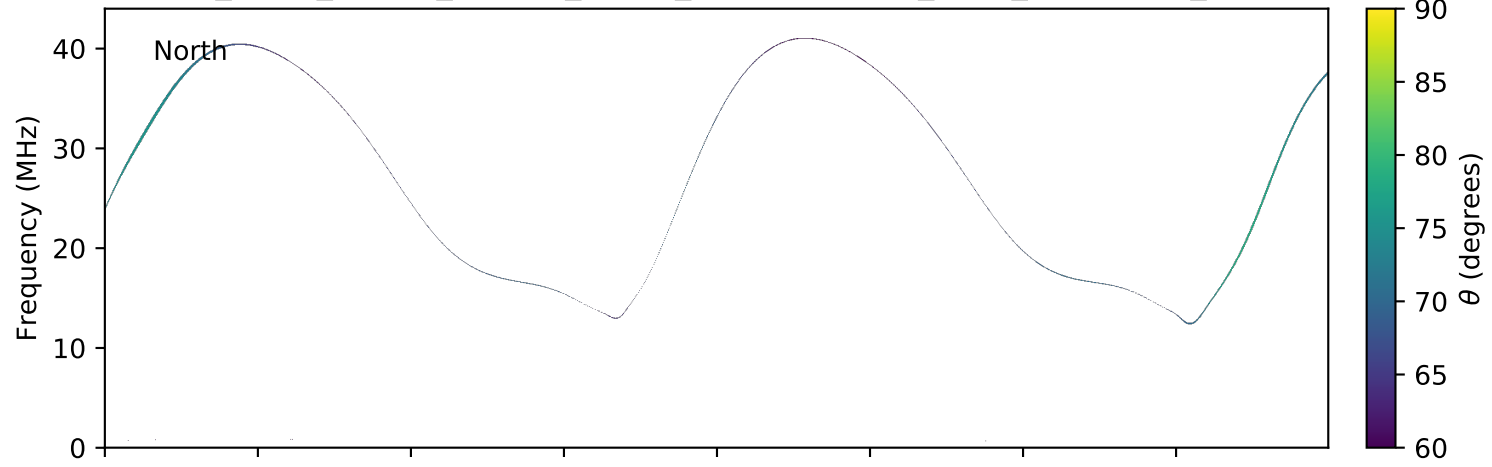
expres_earth_jupiter_europa_jrm09_lossc-wid1deg_3kev_20090302_v01.cdf
