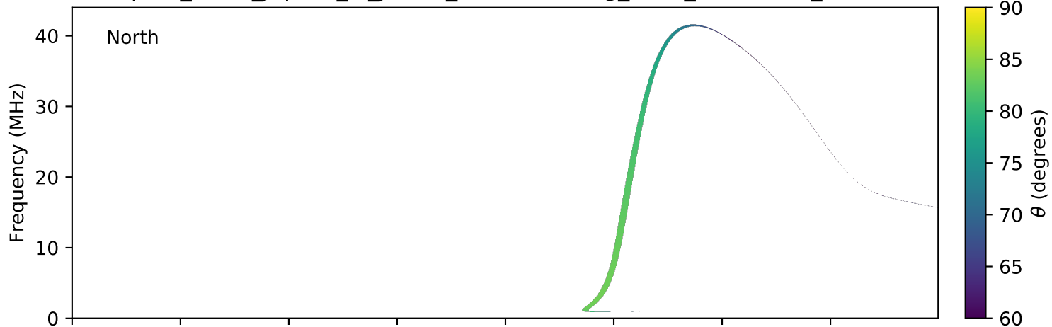
expres_earth_jupiter_io_jrm09_lossc-wid1deg_3kev_20090224_v01.cdf
