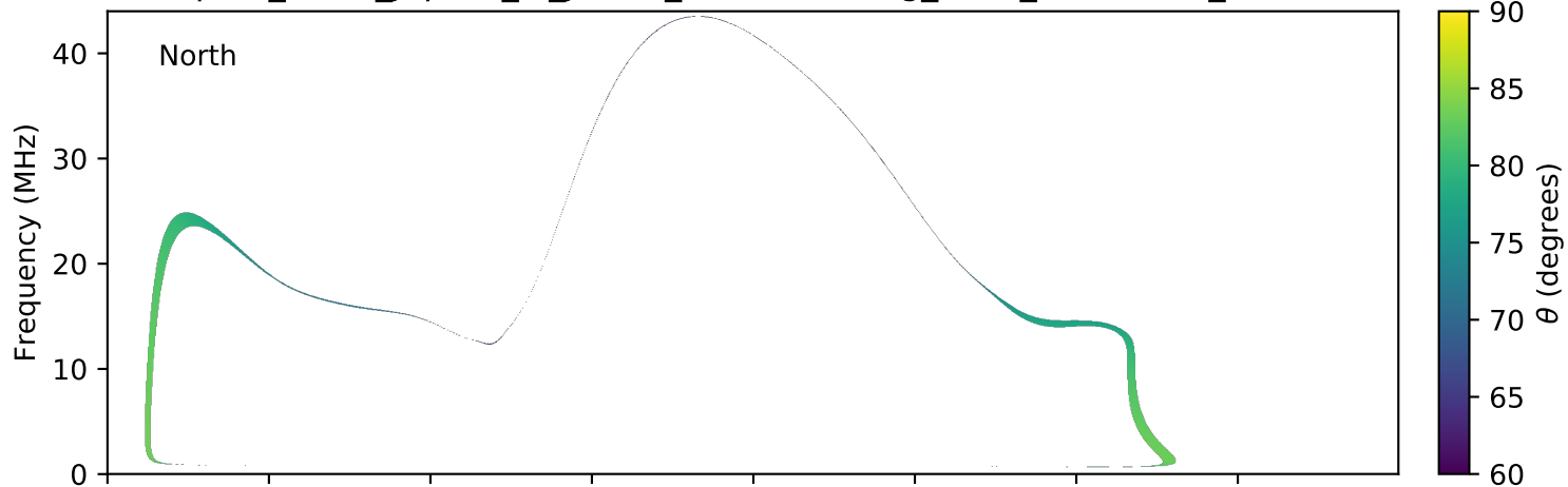
expres_earth_jupiter_io_jrm09_lossc-wid1deg_3kev_20090221_v01.cdf
