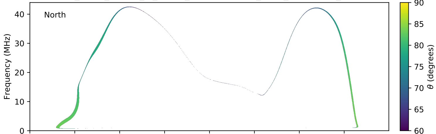
expres_earth_jupiter_io_jrm09_lossc-wid1deg_3kev_20090205_v01.cdf
