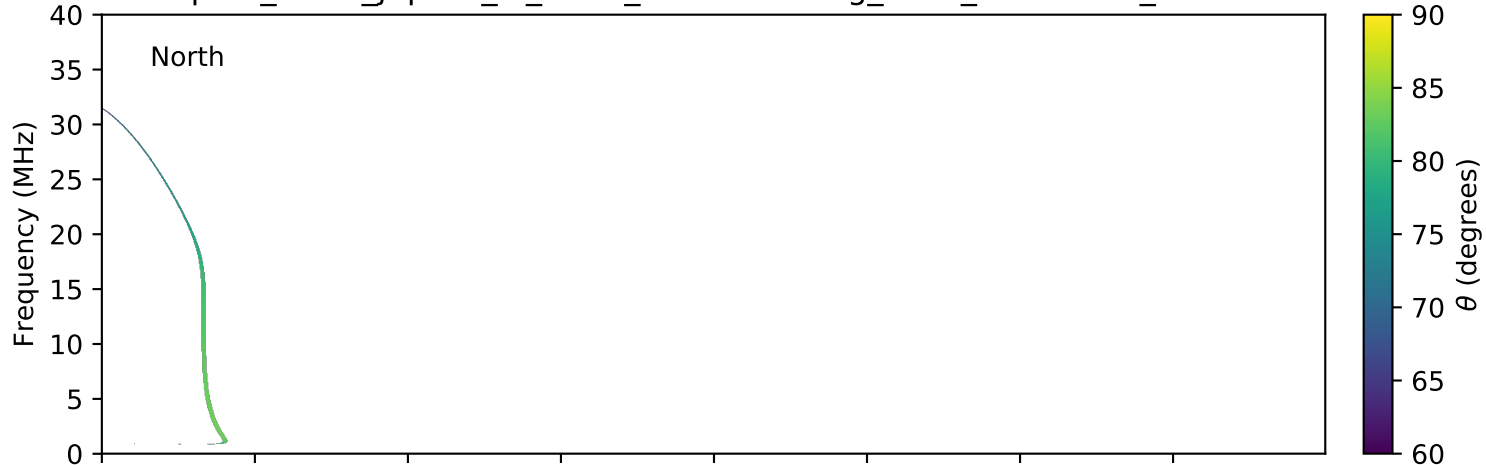
expres_earth_jupiter_io_isaac_lossc-wid1deg_3kev_20090227_v01.cdf
