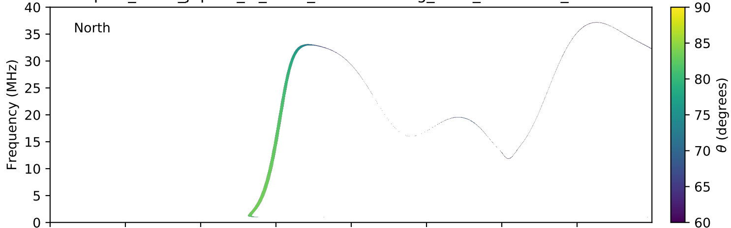
expres_earth_jupiter_io_isaac_lossc-wid1deg_3kev_20090226_v01.cdf
