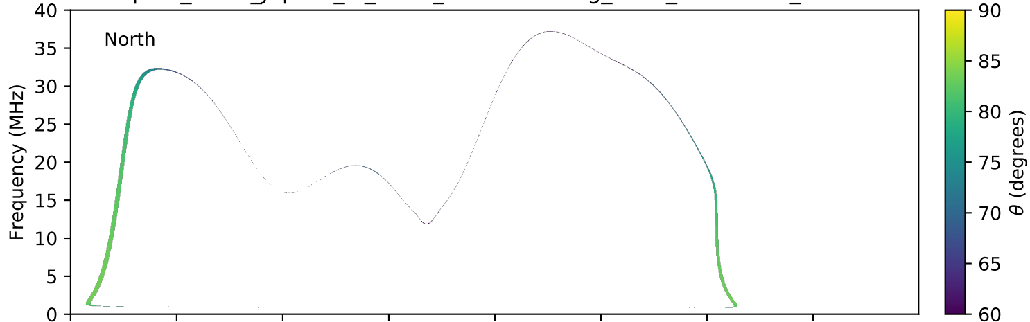
expres_earth_jupiter_io_isaac_lossc-wid1deg_3kev_20090221_v01.cdf
