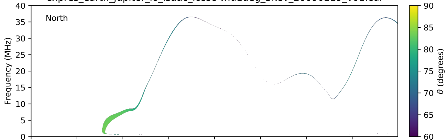
expres_earth_jupiter_io_isaac_lossc-wid1deg_3kev_20090219_v01.cdf
