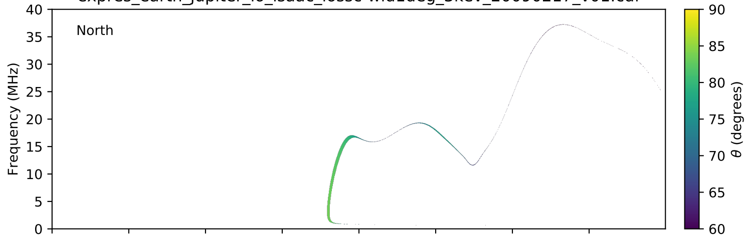
expres_earth_jupiter_io_isaac_lossc-wid1deg_3kev_20090217_v01.cdf
