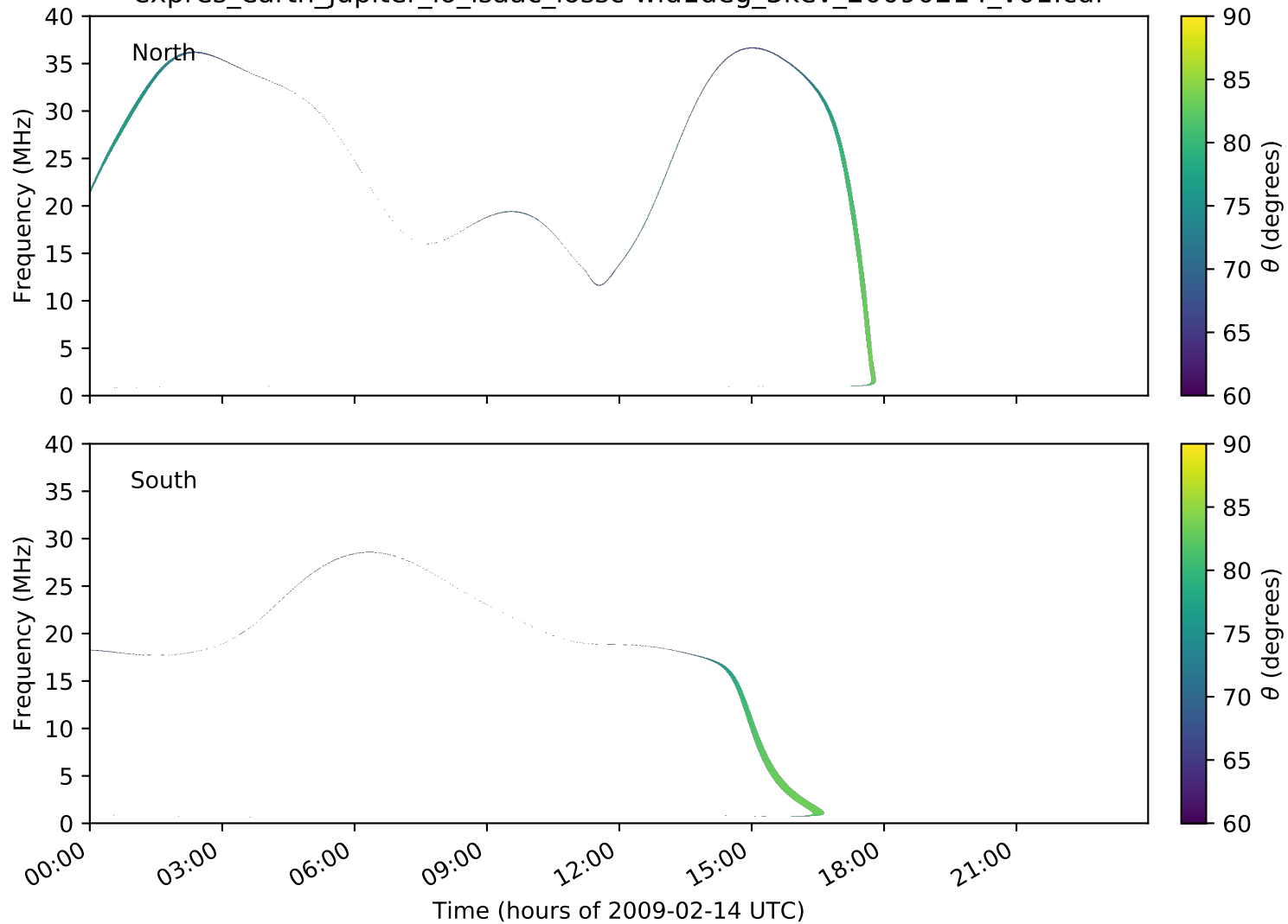
expres_earth_jupiter_io_isaac_lossc-wid1deg_3kev_20090214_v01.cdf
