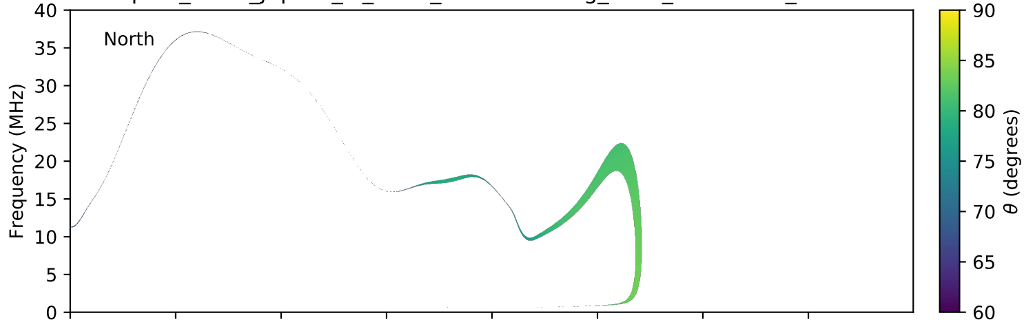
expres_earth_jupiter_io_isaac_lossc-wid1deg_3kev_20090207_v01.cdf
