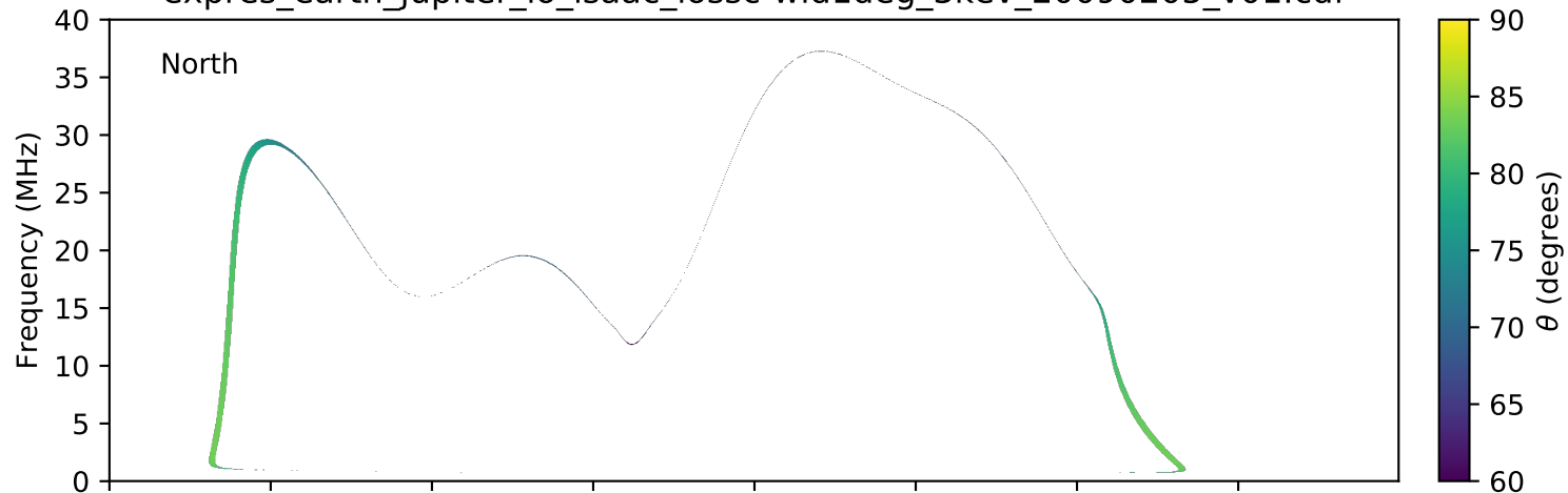
expres_earth_jupiter_io_isaac_lossc-wid1deg_3kev_20090205_v01.cdf
