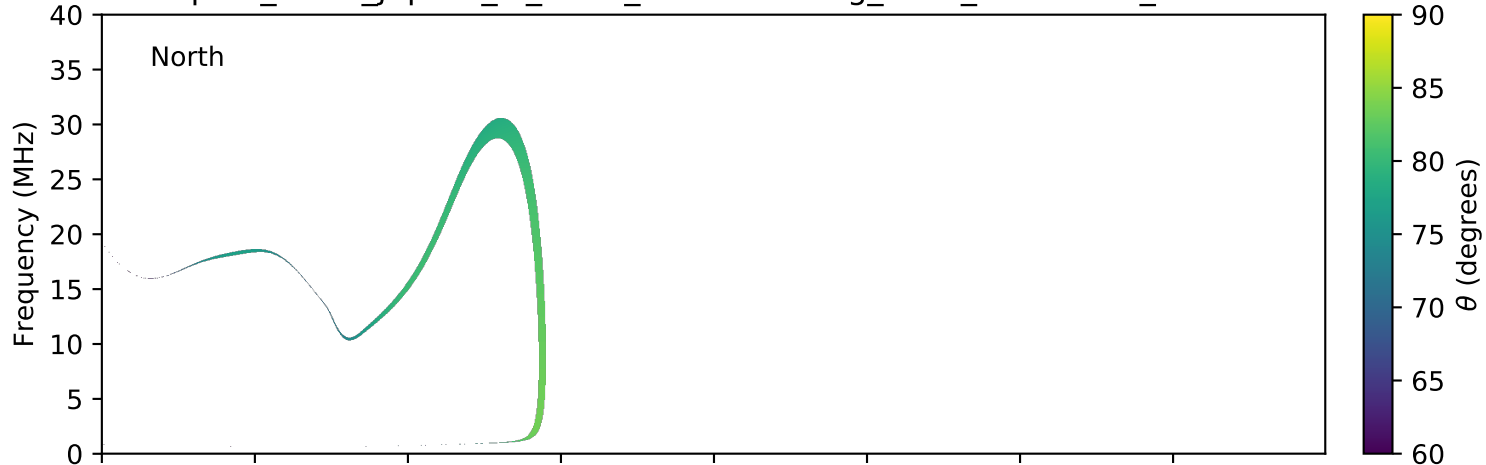
expres_earth_jupiter_io_isaac_lossc-wid1deg_3kev_20090202_v01.cdf
