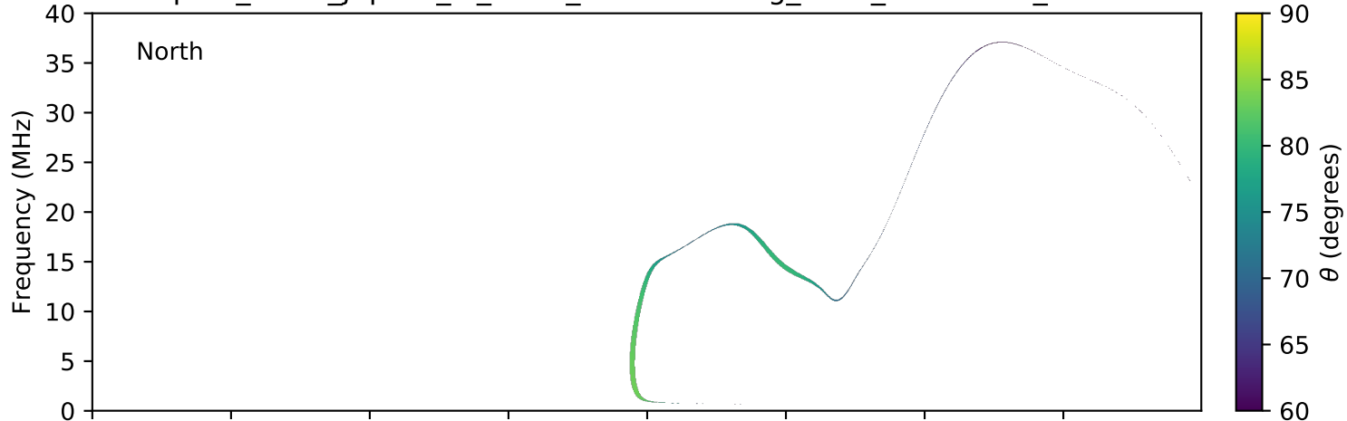
expres_earth_jupiter_io_isaac_lossc-wid1deg_3kev_20090201_v01.cdf
