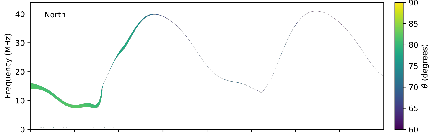
expres_earth_jupiter_europa_jrm09_lossc-wid1deg_3kev_20090219_v01.cdf
