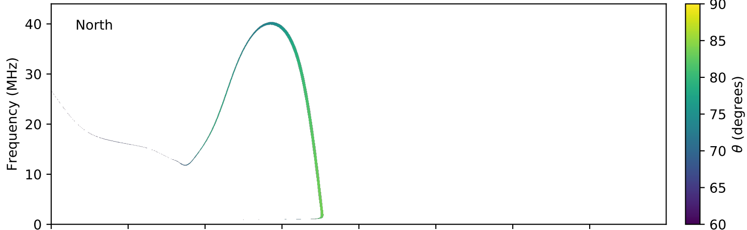
expres_earth_jupiter_io_jrm09_lossc-wid1deg_3kev_20090117_v01.cdf
