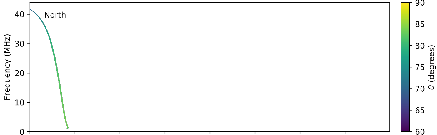
expres_earth_jupiter_io_jrm09_lossc-wid1deg_3kev_20090112_v01.cdf
