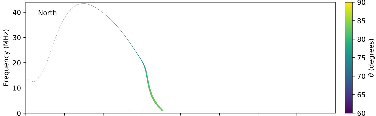
expres_earth_jupiter_io_jrm09_lossc-wid1deg_3kev_20090101_v01.cdf
