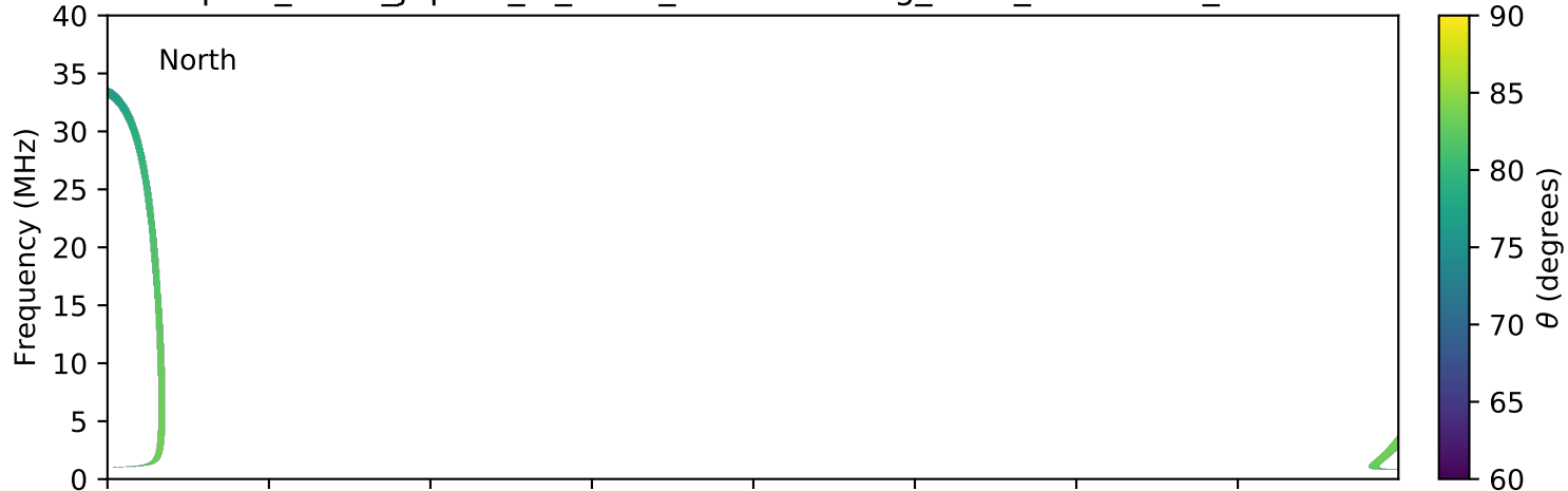
expres_earth_jupiter_io_isaac_lossc-wid1deg_3kev_20090128_v01.cdf
