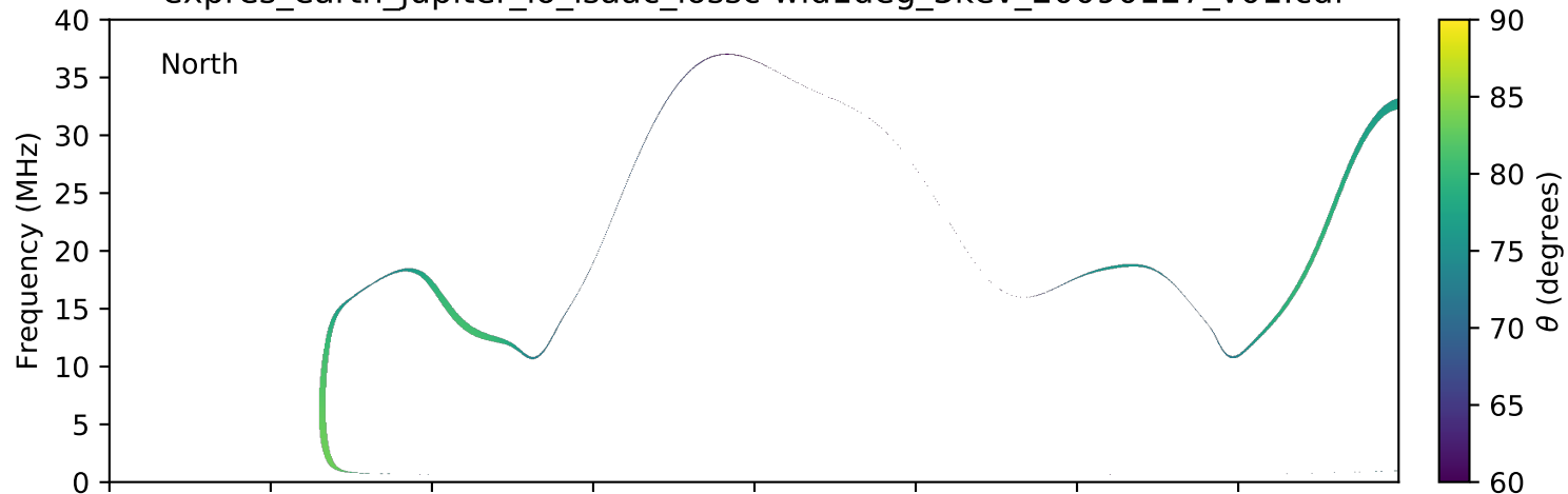
expres_earth_jupiter_io_isaac_lossc-wid1deg_3kev_20090127_v01.cdf
