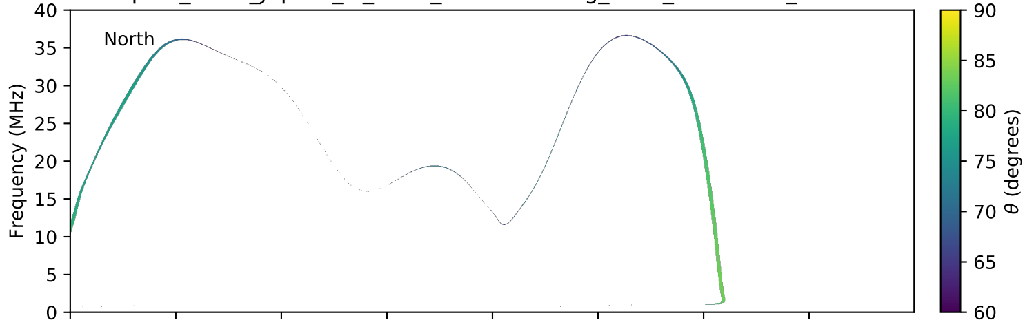
expres_earth_jupiter_io_isaac_lossc-wid1deg_3kev_20090106_v01.cdf
