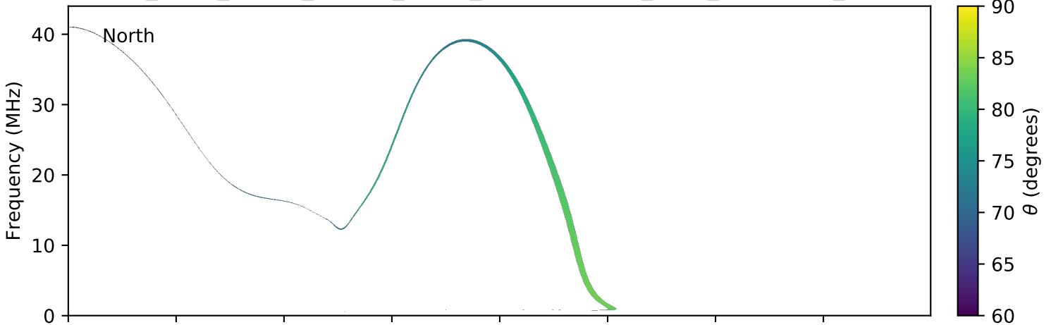
expres_earth_jupiter_europa_jrm09_lossc-wid1deg_3kev_20090126_v01.cdf
