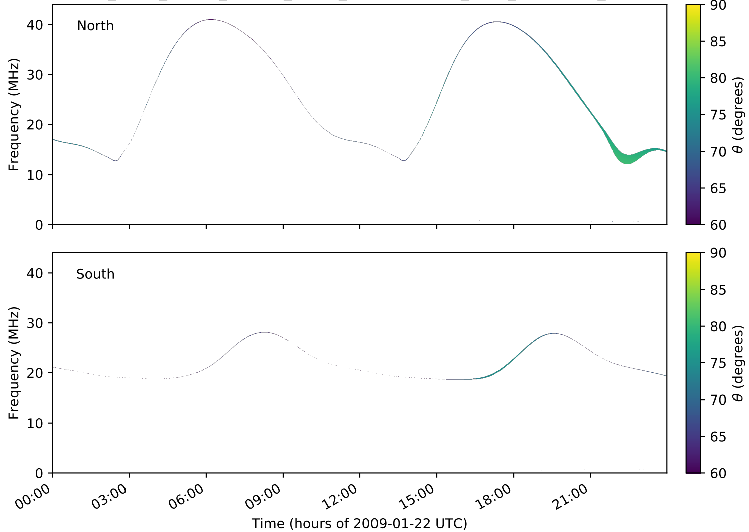
expres_earth_jupiter_europa_jrm09_lossc-wid1deg_3kev_20090122_v01.cdf
