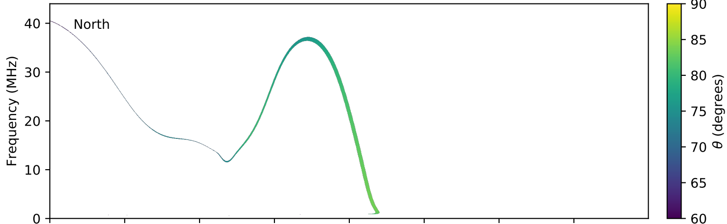
expres_earth_jupiter_europa_jrm09_lossc-wid1deg_3kev_20090119_v01.cdf
