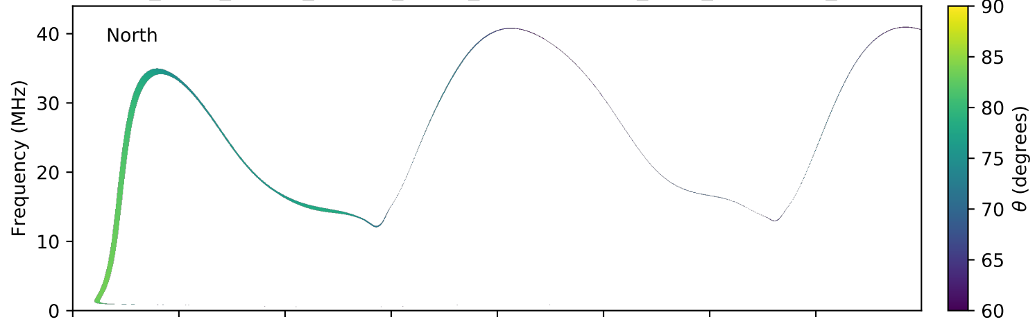
expres_earth_jupiter_europa_jrm09_lossc-wid1deg_3kev_20090118_v01.cdf
