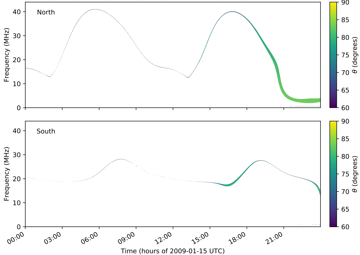
expres_earth_jupiter_europa_jrm09_lossc-wid1deg_3kev_20090115_v01.cdf
