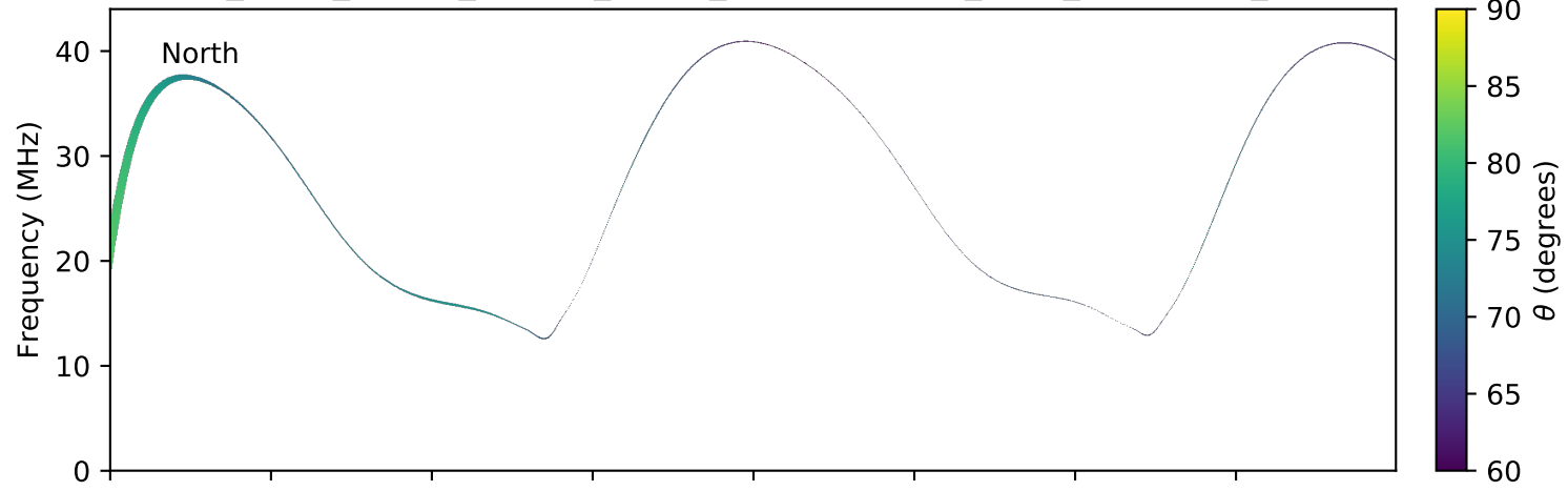
expres_earth_jupiter_europa_jrm09_lossc-wid1deg_3kev_20090111_v01.cdf
