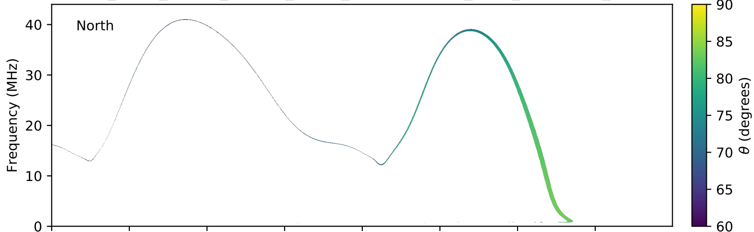
expres_earth_jupiter_europa_jrm09_lossc-wid1deg_3kev_20090108_v01.cdf
