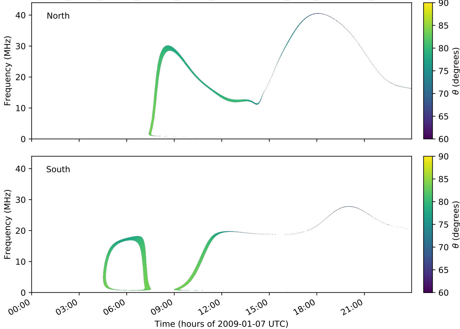
expres_earth_jupiter_europa_jrm09_lossc-wid1deg_3kev_20090107_v01.cdf
