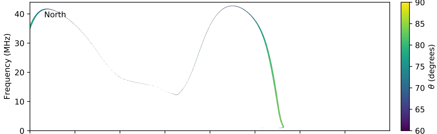
expres_earth_jupiter_io_jrm09_lossc-wid1deg_3kev_20081230_v01.cdf
