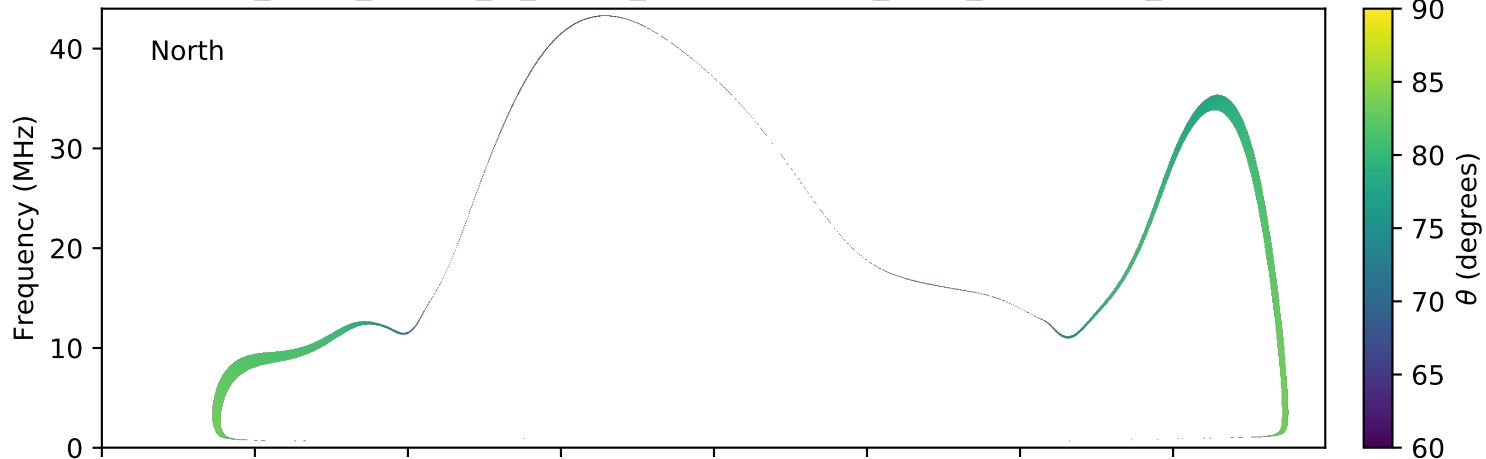
expres_earth_jupiter_io_jrm09_lossc-wid1deg_3kev_20081228_v01.cdf
