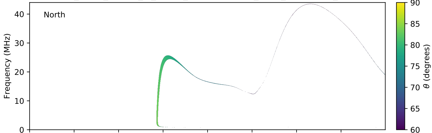
expres_earth_jupiter_io_jrm09_lossc-wid1deg_3kev_20081226_v01.cdf
