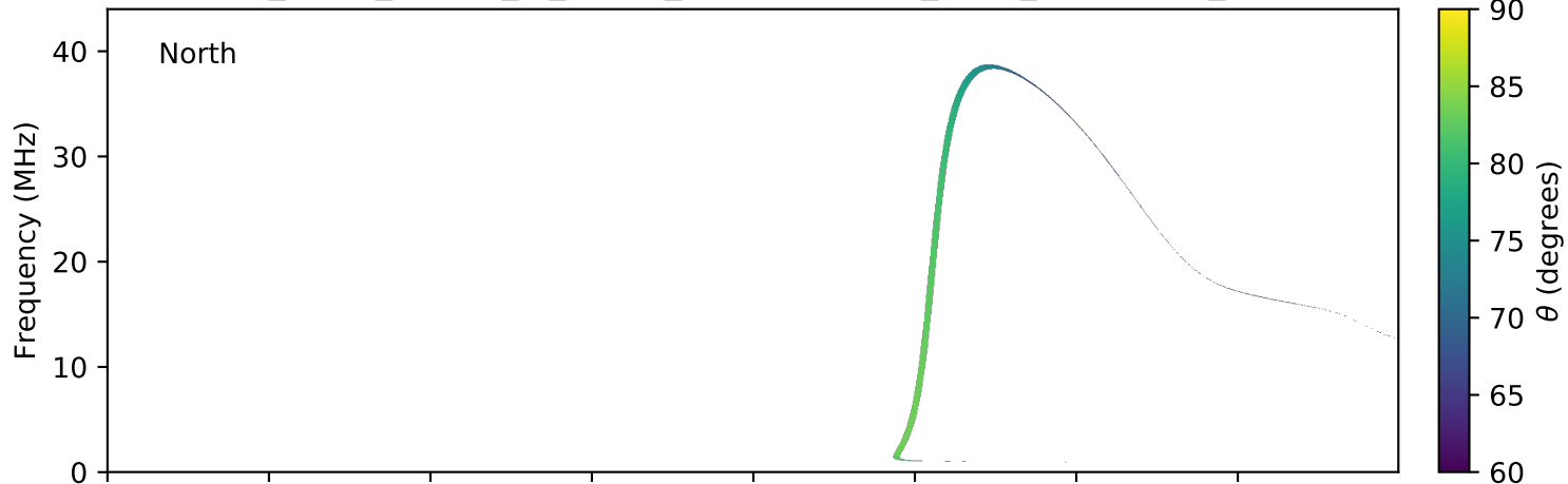
expres_earth_jupiter_io_jrm09_lossc-wid1deg_3kev_20081224_v01.cdf
