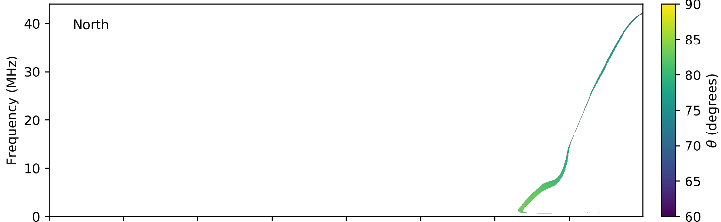
expres_earth_jupiter_io_jrm09_lossc-wid1deg_3kev_20081222_v01.cdf
