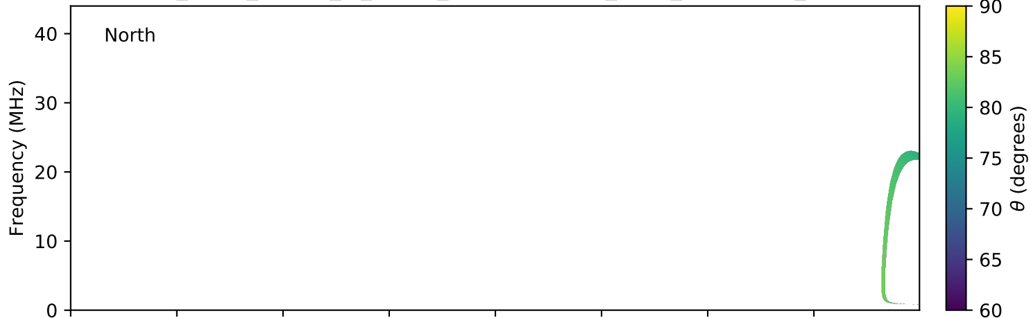
expres_earth_jupiter_io_jrm09_lossc-wid1deg_3kev_20081213_v01.cdf
