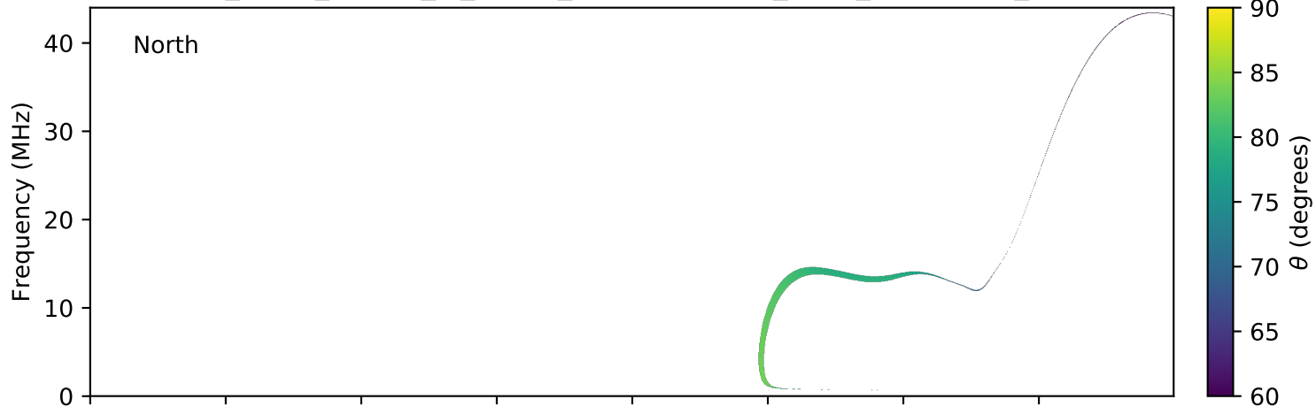
expres_earth_jupiter_io_jrm09_lossc-wid1deg_3kev_20081208_v01.cdf
