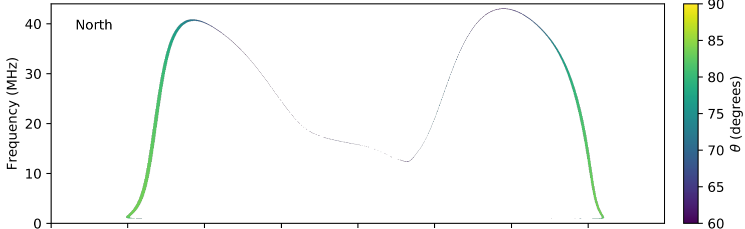
expres_earth_jupiter_io_jrm09_lossc-wid1deg_3kev_20081205_v01.cdf
