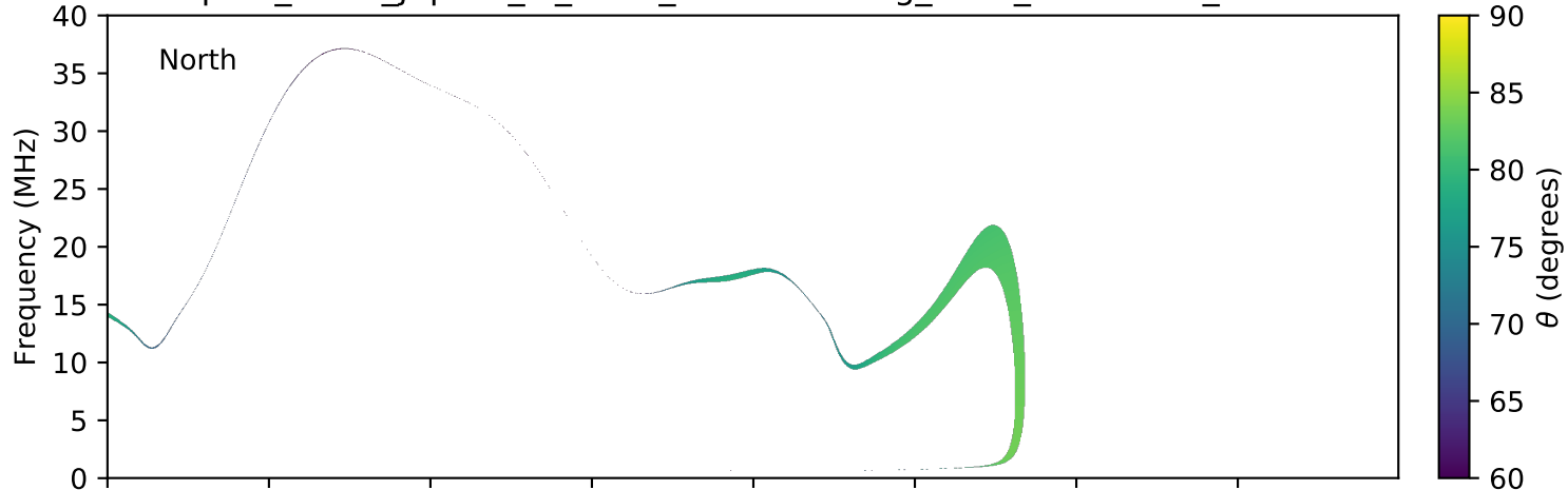
expres_earth_jupiter_io_isaac_lossc-wid1deg_3kev_20081230_v01.cdf
