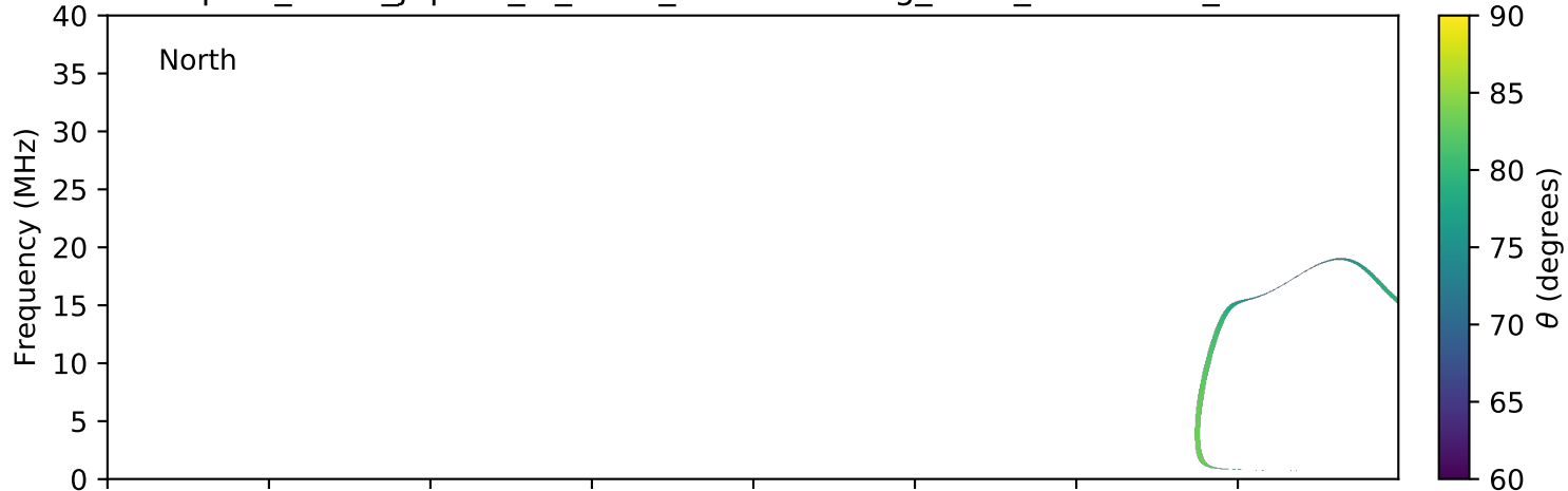
expres_earth_jupiter_io_isaac_lossc-wid1deg_3kev_20081229_v01.cdf
