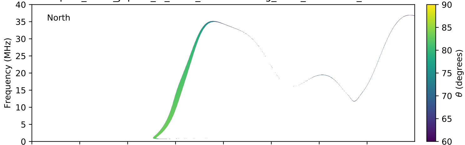
expres_earth_jupiter_io_isaac_lossc-wid1deg_3kev_20081226_v01.cdf
